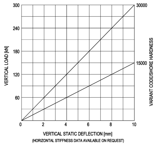
LOAD CHARACTERISTICS
