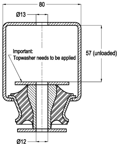
CROSS-SECTION
